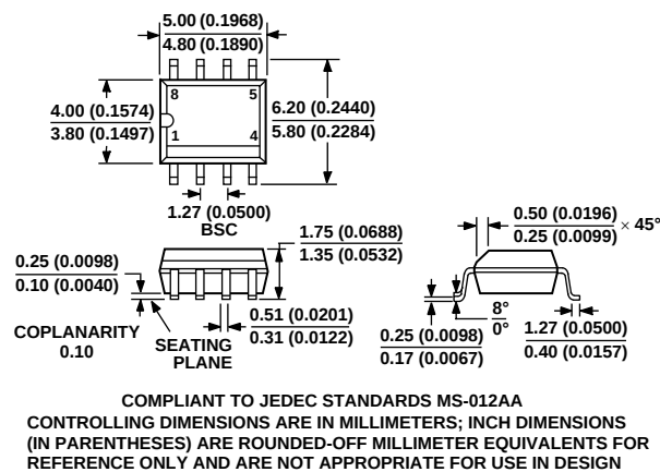
Figure 9. 8-Lead Standard Small Outline Package [SOIC]—Narrow Body (R-8) Dimensions shown in millimeters (inches)
