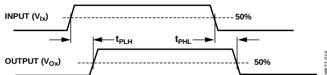
Figure 26. Propagation Delay Parameters
