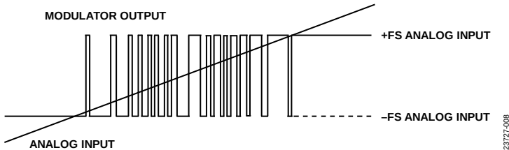
Figure 26. Analog Input vs. Modulator Output
