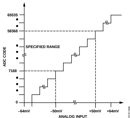
Figure 27. Filtered and Decimated 16-Bit Transfer Function
