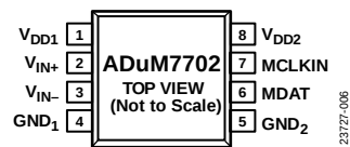
Figure 6. 8-Lead SOIC_IC Pin Configuration
