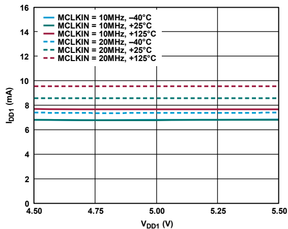
Figure 20. I_{DD1} vs. V_{DD1} at Clock Rates and Various Temperatures
