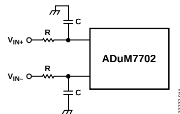
Figure 29. RC Low-Pass Filter Input Network
