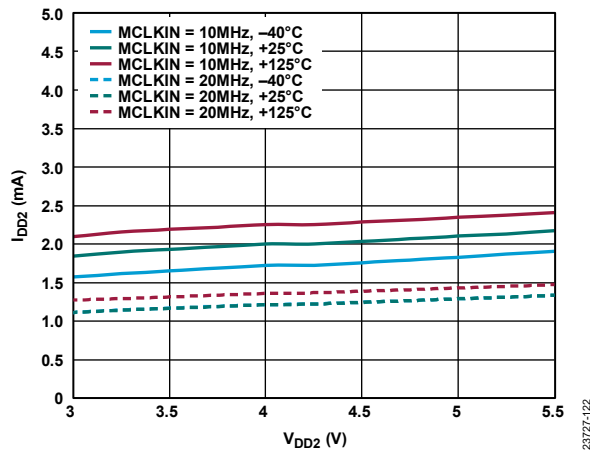
Figure 22. I_{DD2} vs. V_{DD2} at Various Clock Rates and Temperatures
