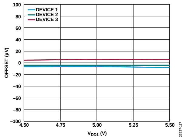
Figure 17. Offset vs. V_{DD1}
