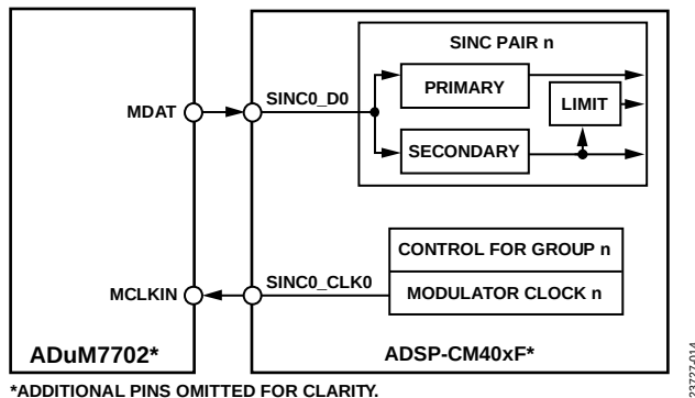
Figure 32. Interfacing the ADuM7702 to the ADSP-CM4xx
