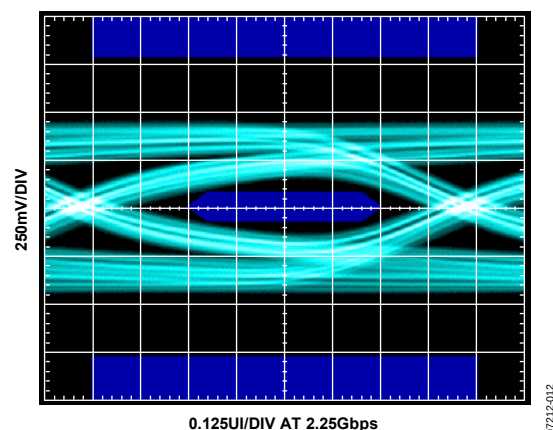
Figure 12. Tx Eye Diagram at TP3, PE = 0 dB (Cable = 6 Meters, 24 AWG)
