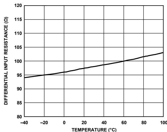
Figure 24. Differential Input Resistance vs. Temperature
