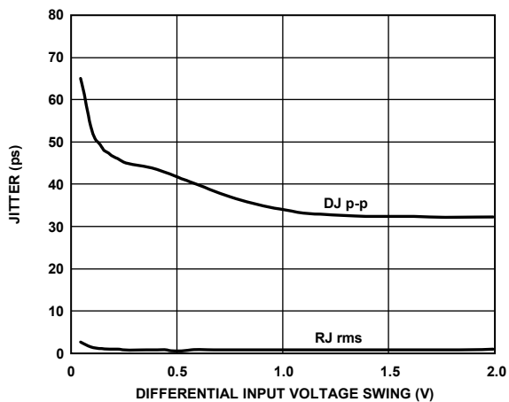
Figure 20. Jitter vs. Differential Input Voltage Swing
