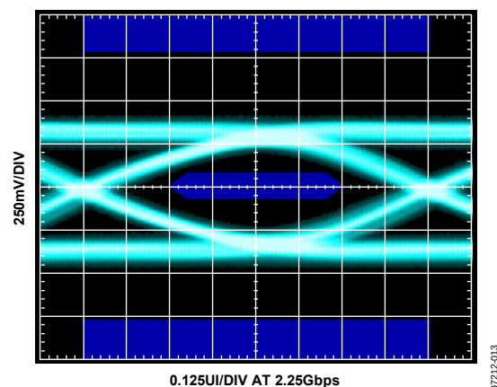
Figure 13. Tx Eye Diagram at TP3, PE = 6 dB (Cable = 10 Meters, 24 AWG)
