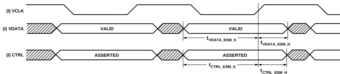
Figure 27. Multiplexed Philips Video—Encode and Slave Pixel (YCrCb) Transfer Timing
