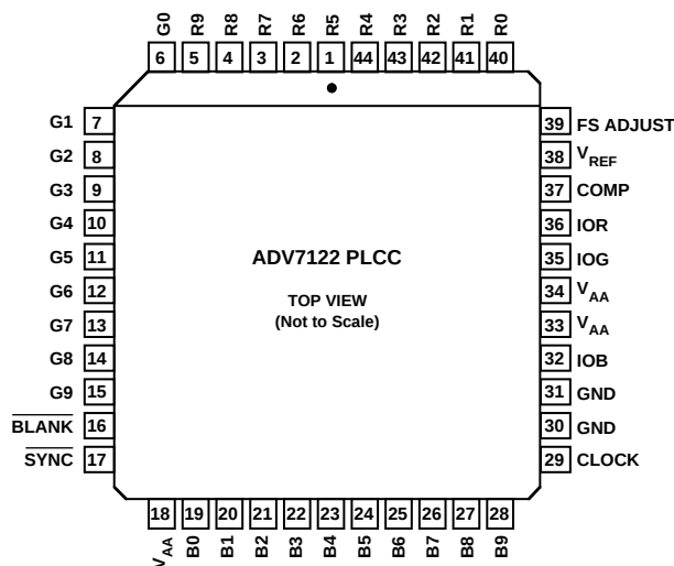
PLCC (P-44A) Package
