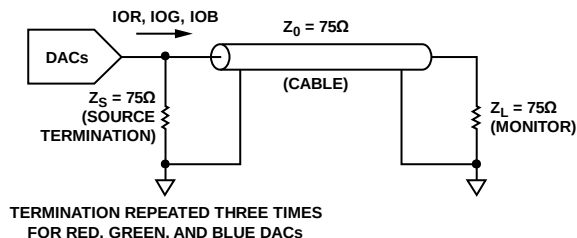
Figure 24. Analog Output Termination for RS-343A
