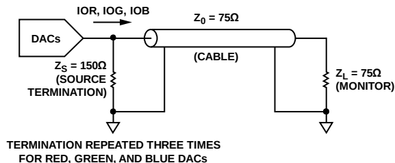
Figure 25. Analog Output Termination for RS-170
