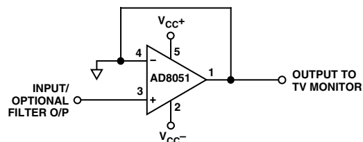
Figure 95. Recommended Output DAC Buffer
