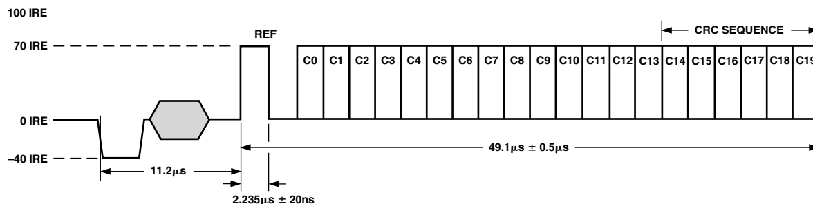
Figure 70. CGMS Waveform Diagram
