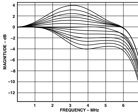
Figure 21. Extended Mode Luma Filter with Programmable Gain, Combined Response
