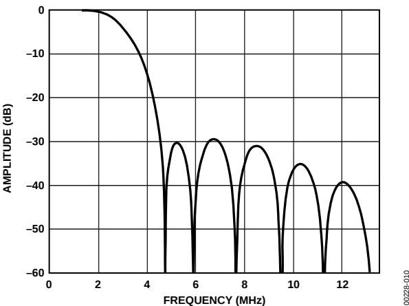
Figure 10. PAL Notch Filter
