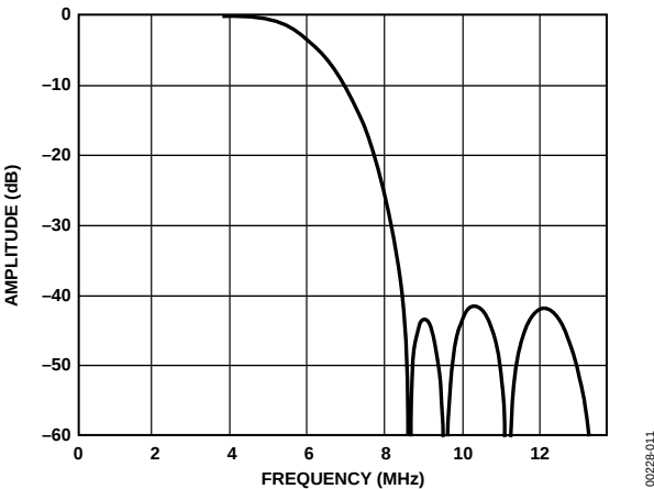
Figure 11. NTSC/PAL Extended Mode Filter
