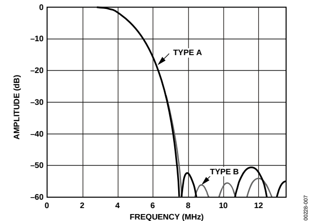
Figure 7. NTSC Low-Pass Filter
