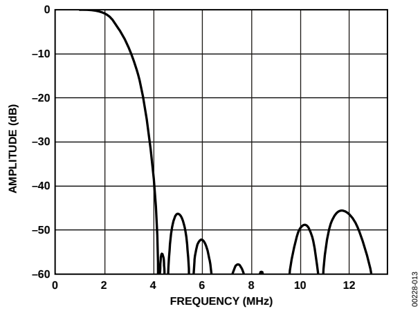
Figure 13 . PAL UV Filter
