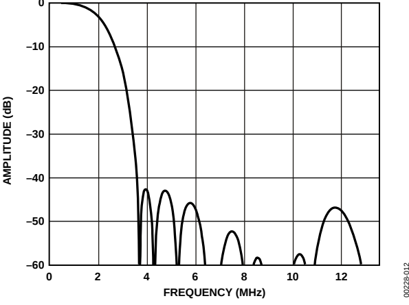
Figure 12. NTSC UV Filter
