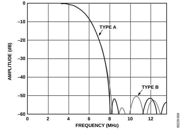
Figure 9. PAL Low-Pass Filter
