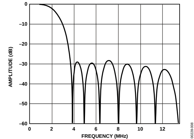
Figure 8. NTSC Notch Filter
