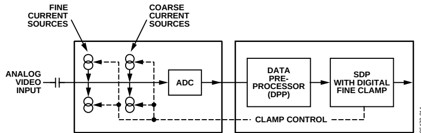
Figure 14. Clamping Overview
