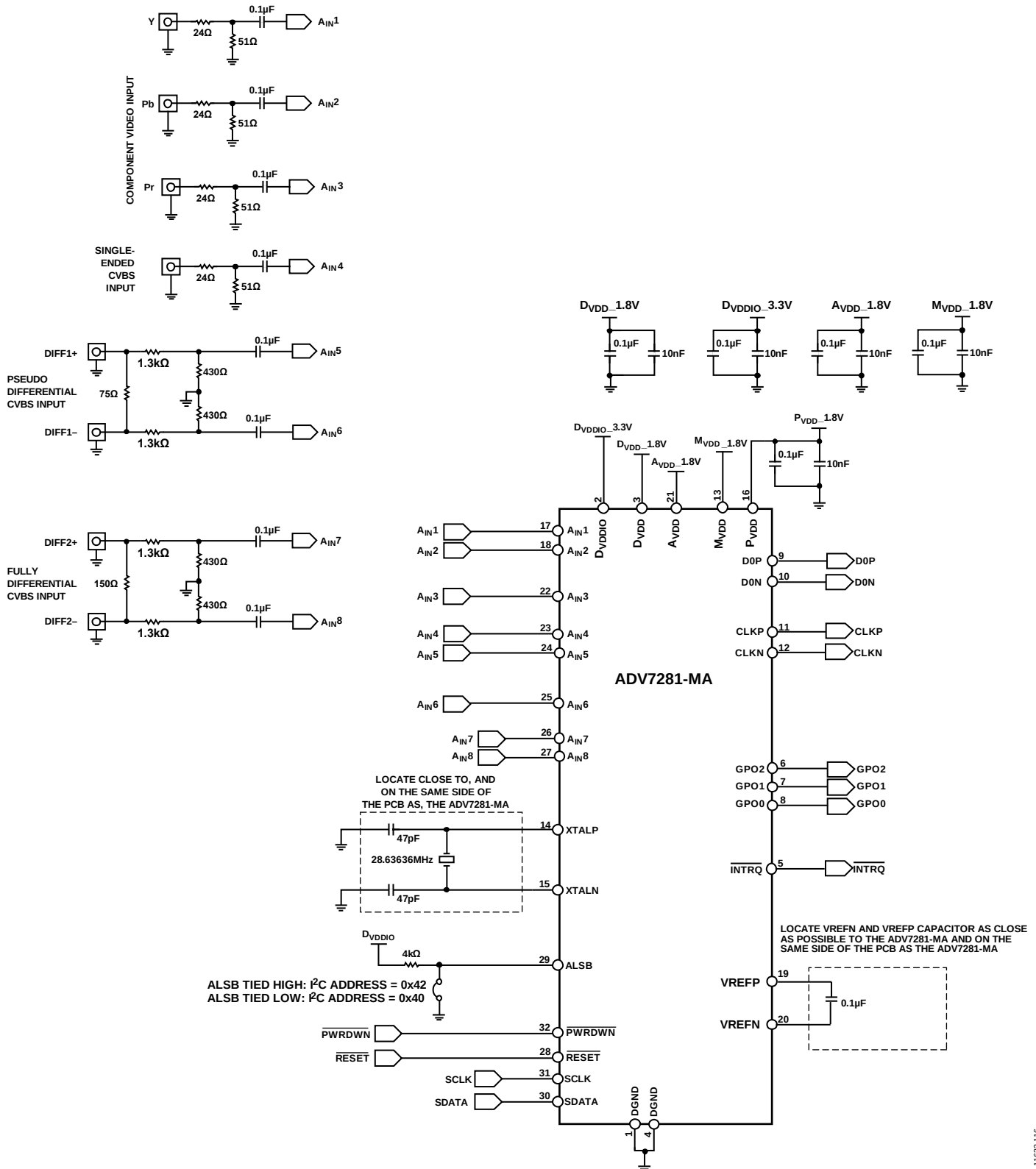
Figure 17. Typical Connection Diagram, ADV7281-MA
