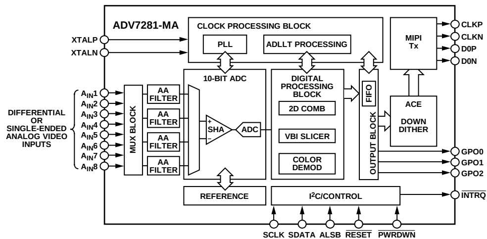
Figure 2. ADV7281-MA Functional Block Diagram
