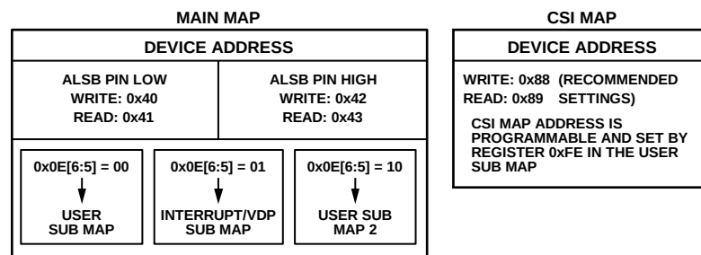
Figure 14. Register Map and Sub Map Access
