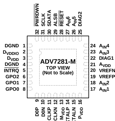
Figure 5. Pin Configuration, ADV7281-M
