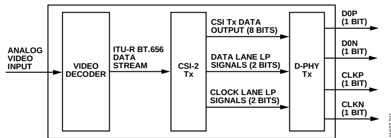
Figure 11. MIPI CSI-2 Output Stage of the ADV7281-M/ADV7281-MA
