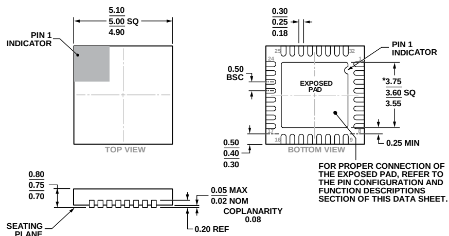
Figure 18. 32-Lead Lead Frame Chip Scale Package [LFCSP_WQ] 5 mm x 5 mm Body, Very Very Thin Quad (CP-32-12) Dimensions shown in millimeters
