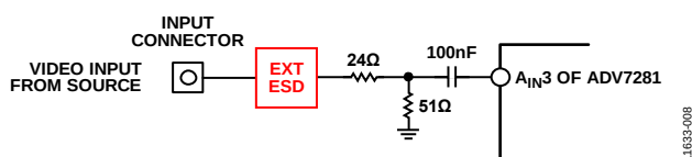
Figure 8. Single-Ended Input Network
