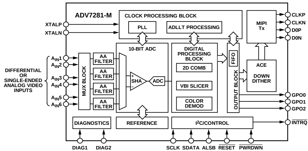
Figure 1. ADV7281-M Functional Block Diagram
