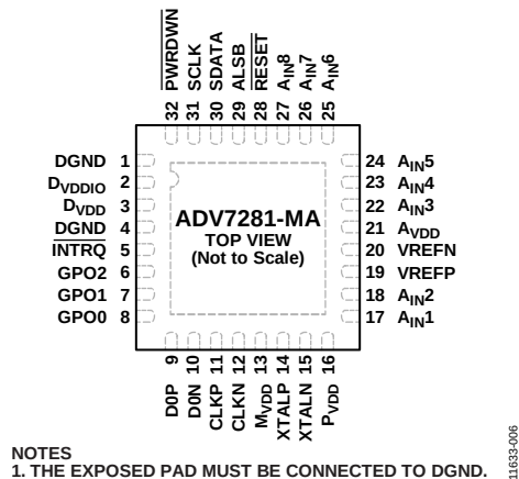
Figure 6. Pin Configuration, ADV7281-MA
