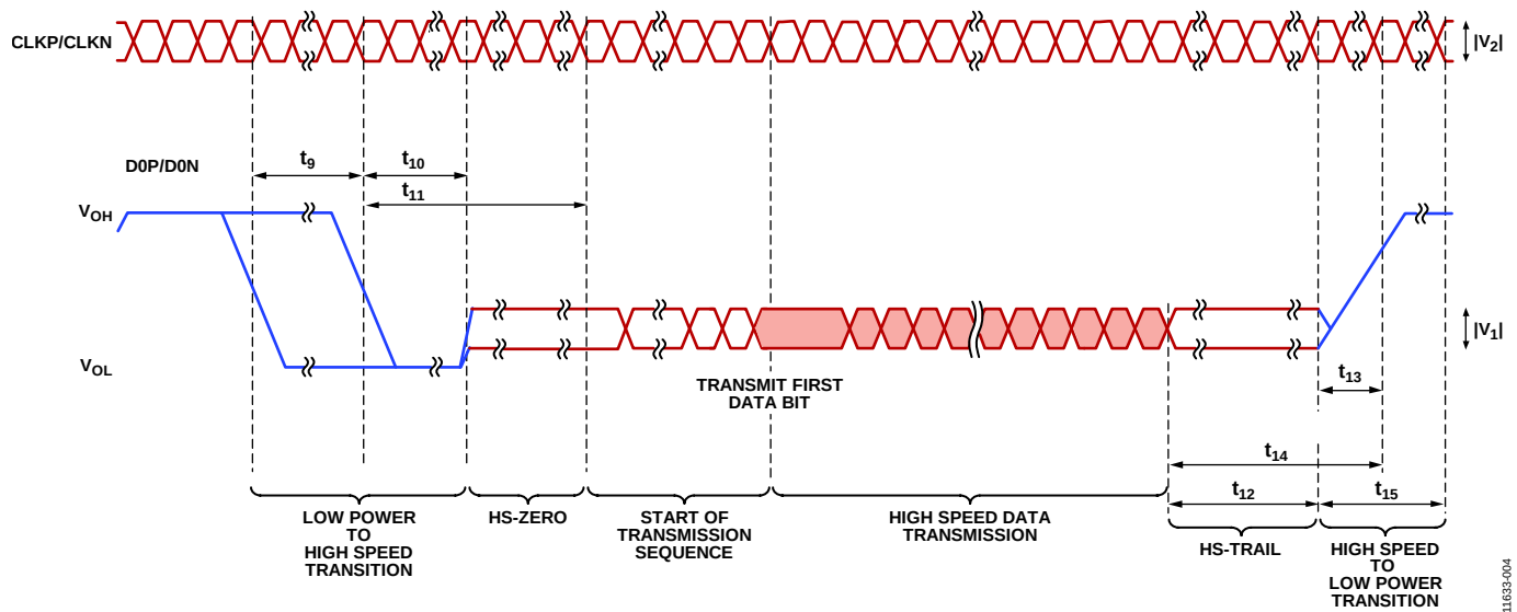
Figure 3. ADV7281-M/ADV7281-MA Output Timing Diagram (Conforms with MIPI CSI-2 Specification)
