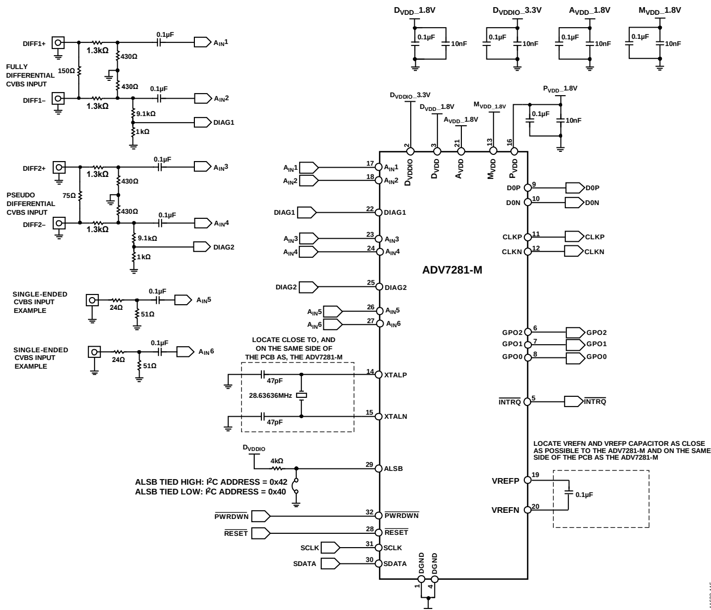
Figure 16. Typical Connection Diagram, ADV7281-M
