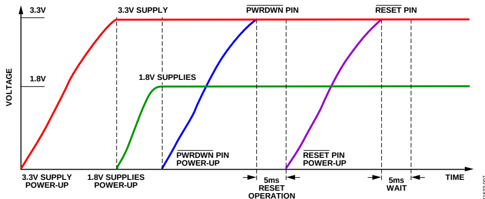
Figure 7. Optimal Power-Up Sequence
