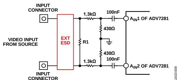
Figure 9. Differential Input Network
