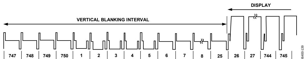
Figure 139. SMPTE 296M (720p)
