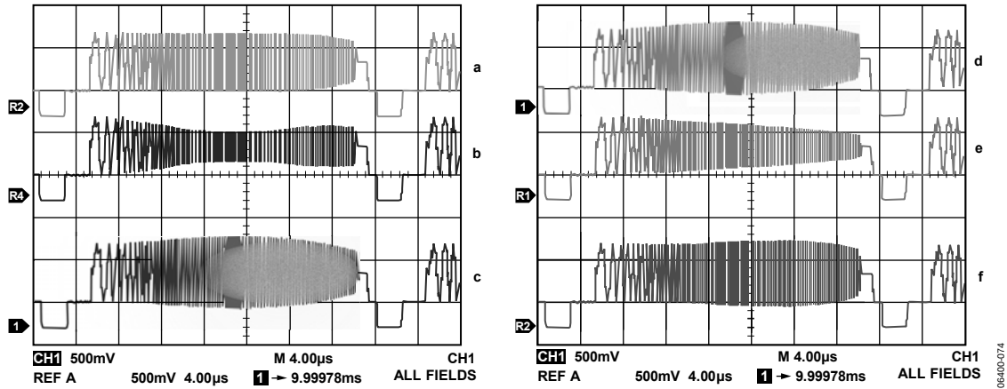
Figure 72. ED/ HD Sharpness Filter Control with Different Gain Settings for ED/HD Sharpness Filter Gain Values
