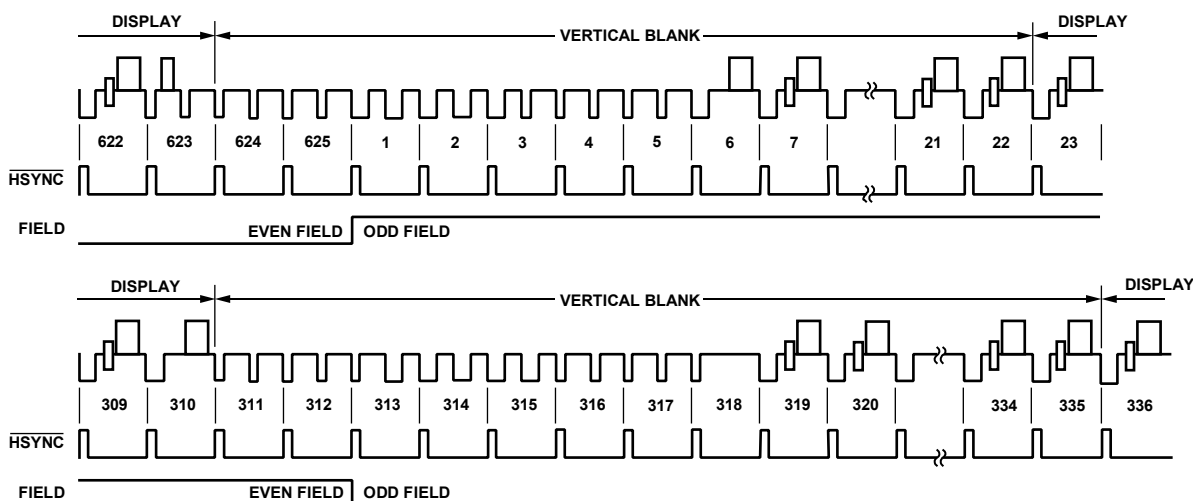
Figure 113. SD Timing Mode 3, PAL
