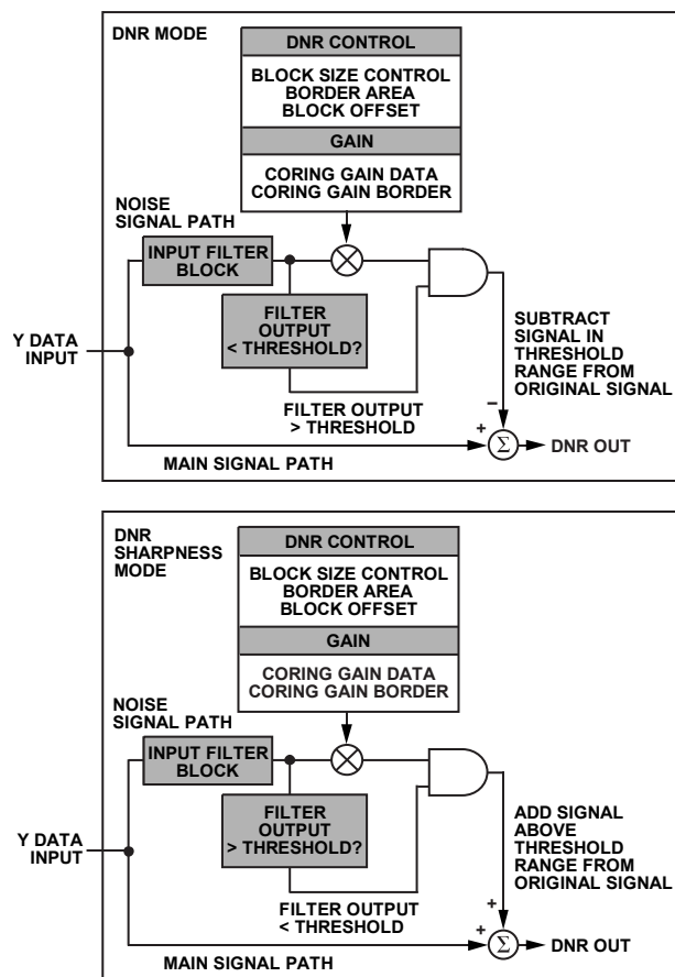
Figure 76. SD DNR Block Diagram
