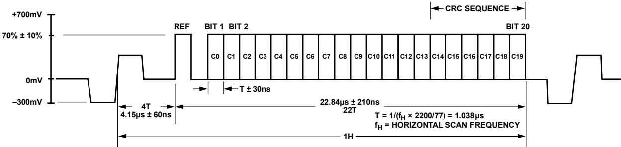
Figure 96. High Definition (1080i) CGMS Waveform
