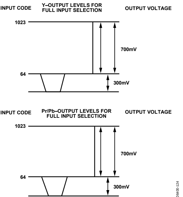
Figure 124. Output Levels for Full Input Selection
