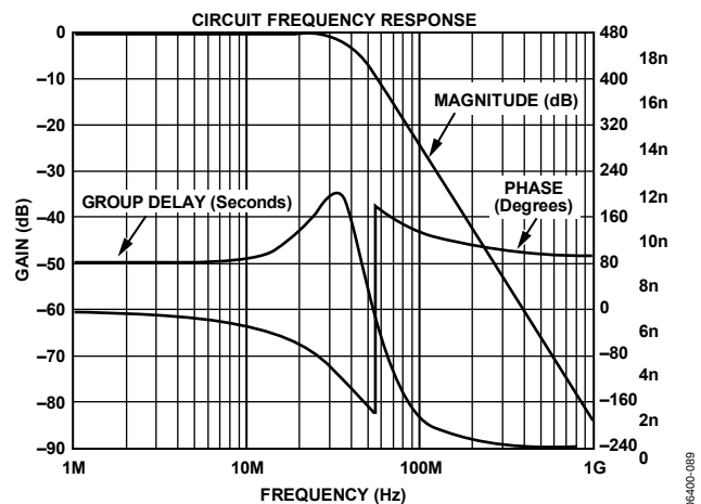
Figure 89. Output Filter Plot for ED, 8x Oversampling
