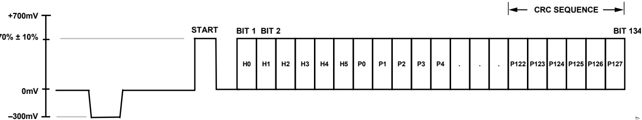
Figure 97. Enhanced Definition (525p) CGMS Type B Waveform
