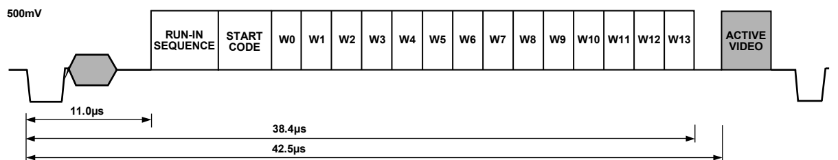
Figure 99. WSS Waveform Diagram
