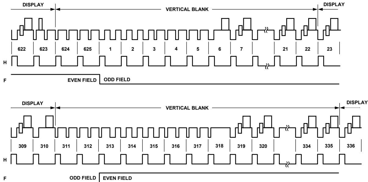
Figure 103. SD Master Mode 0, PAL
