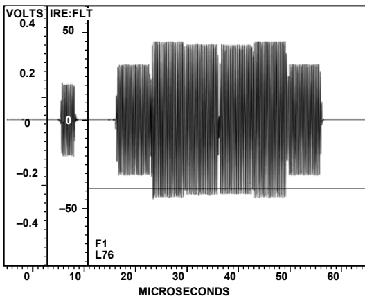
Figure 130. NTSC Luma
