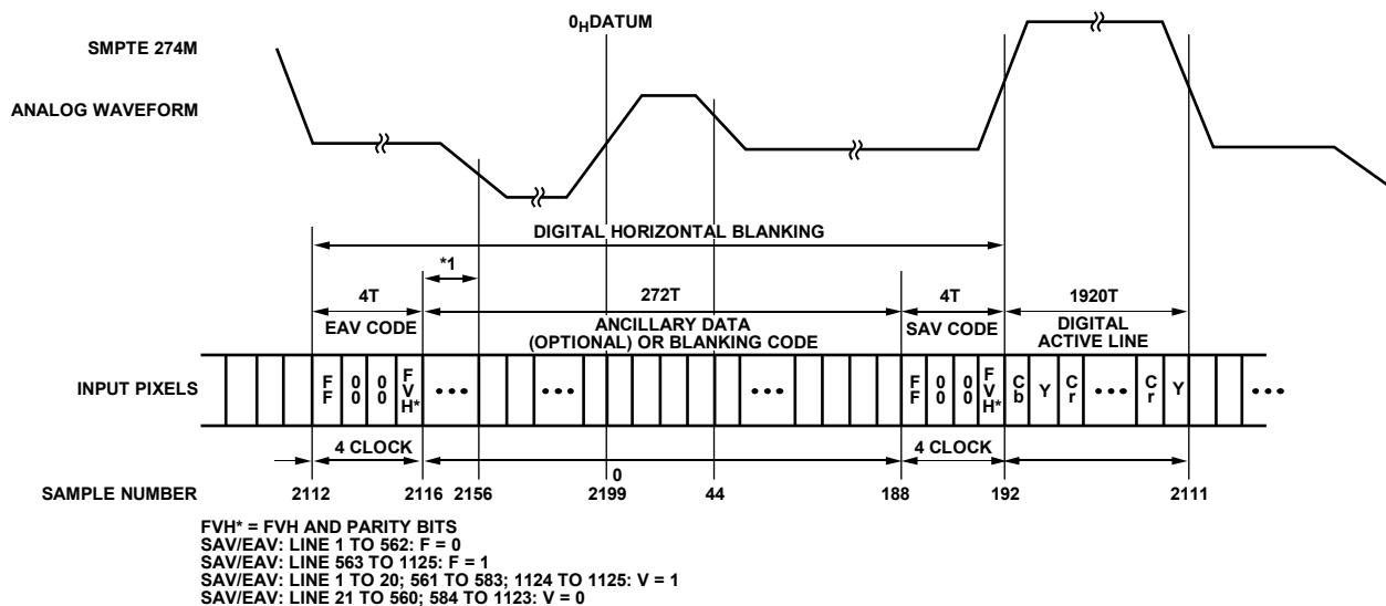
Figure 135. EAV/SAV Input Data Timing Diagram (SMPTE 274M)
