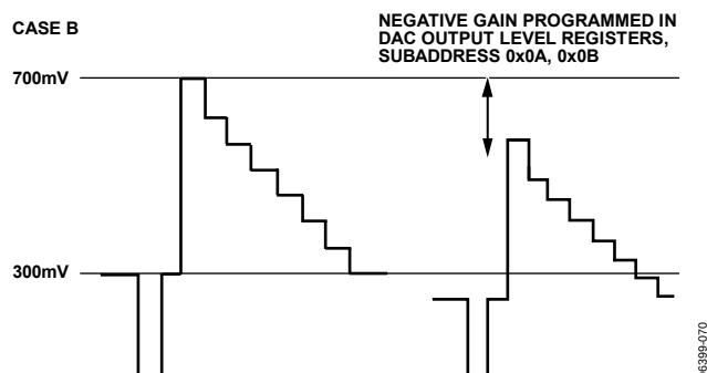
Figure 68. Programmable DAC Gain—Positive and Negative Gain
