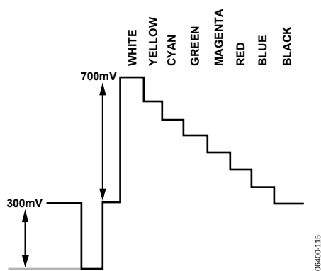
Figure 115. Y Levels—NTSC
