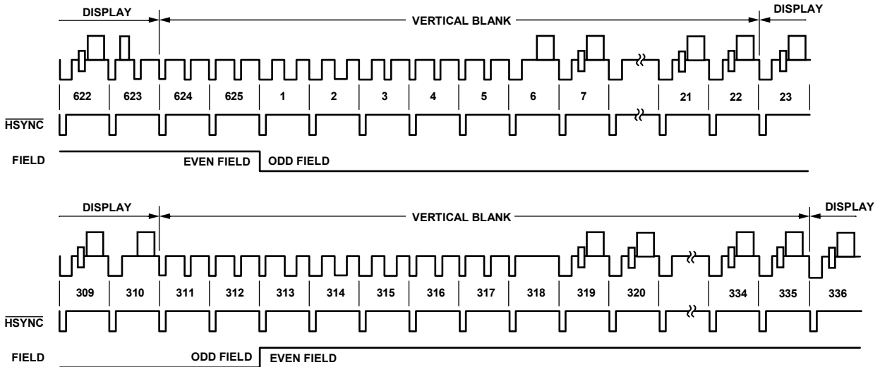
Figure 106. SD Slave Mode 1, PAL
