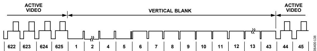
Figure 138. ITU-R BT.1358 (625p)
