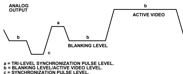
Figure 58. ED/HD Nonstandard Timing Mode Output Levels
