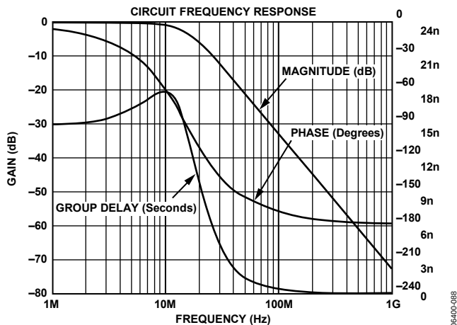
Figure 88. Output Filter Plot for SD, 16x Oversampling
