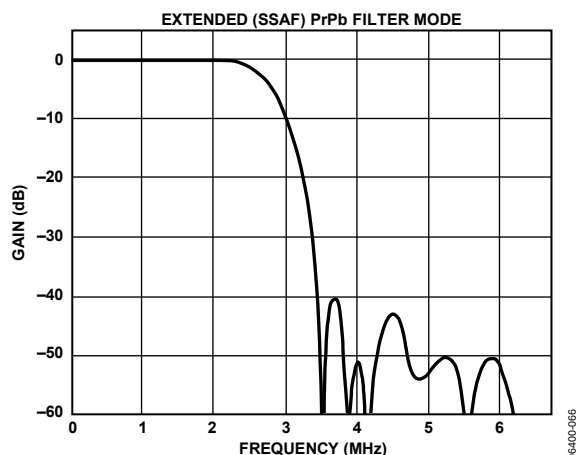
Figure 64. PrPb SSAF Filter
