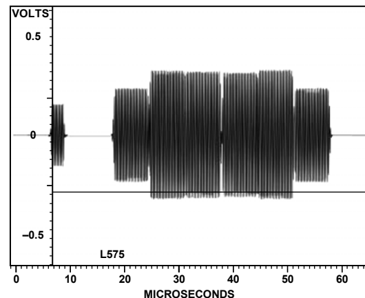
Figure 133. PAL Luma
