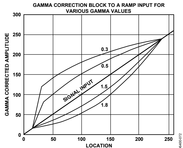
Figure 70. Signal Input (Ramp) and Selectable Output Curves
