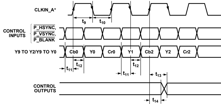
Figure 8. ED/HD-DDR Only, 8-/10-Bit, 4:2:2 YCrCb ( \overline{HSYNC}/\overline{VSYNC} ) Pixel Input Mode (Input Mode 010)
