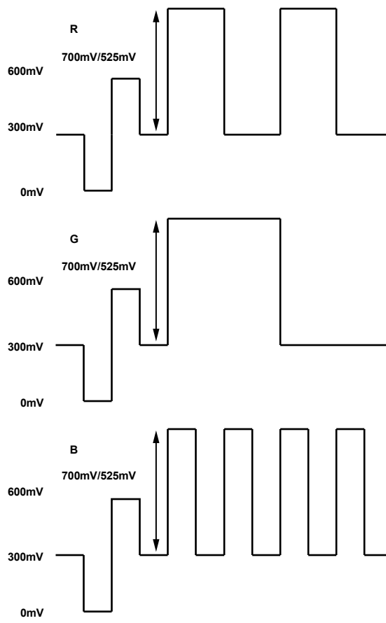
Figure 128. HD RGB Output Levels—RGB Sync Enabled
