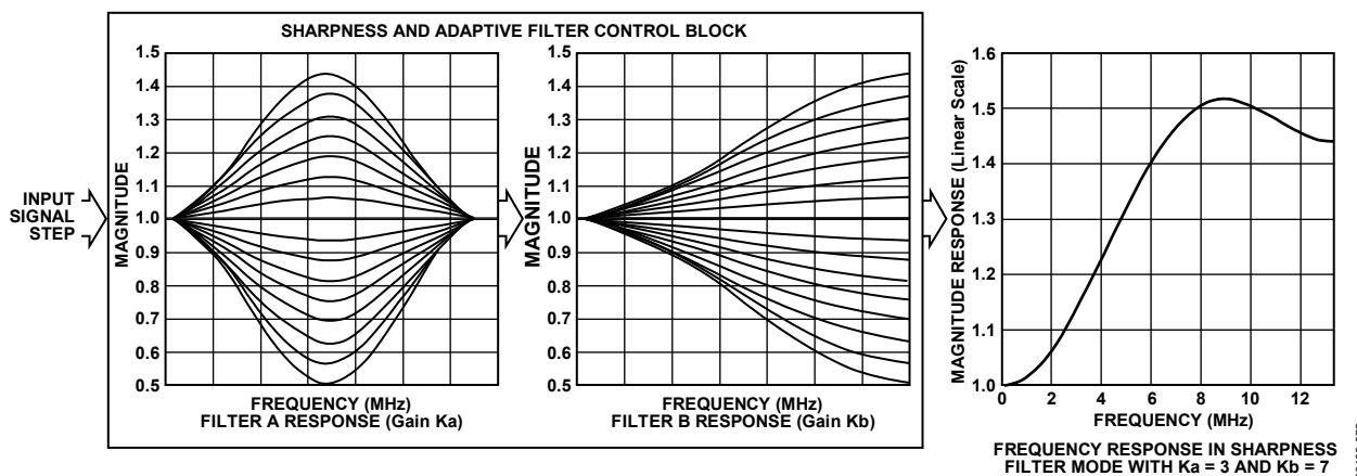
Figure 71. ED/HD Sharpness and Adaptive Filter Control Block
