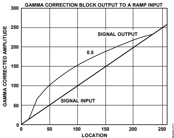
Figure 69. Signal Input (Ramp) and Signal Output for Gamma 0.5
