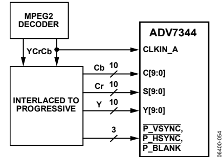
Figure 53. ED/HD Only Example Application
