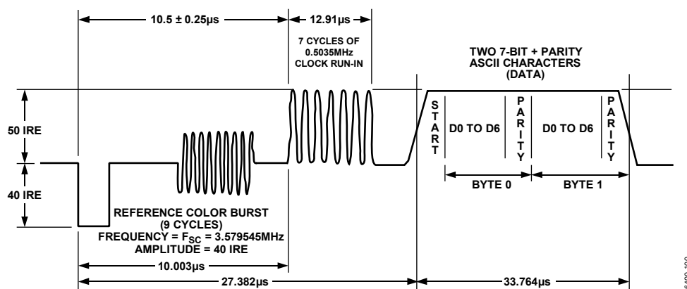
Figure 100. SD Closed Captioning Waveform, NTSC
