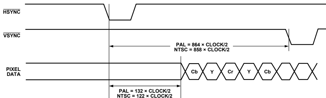
Figure 111. SD Timing Mode 2, Odd-to-Even Field Transition (Master/Slave)
