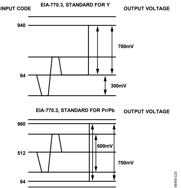
Figure 123. EIA-770.3 Standard Output Signals (1080i/720p)
