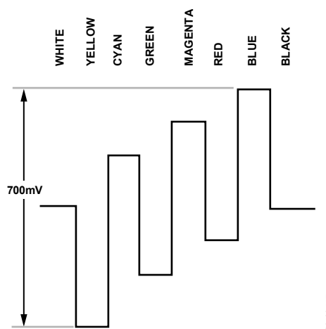
Figure 117. Pb Levels—NTSC
