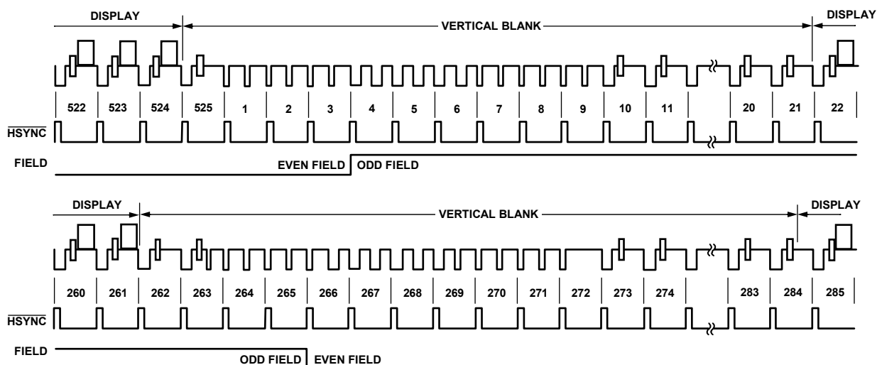
Figure 112. SD Timing Mode 3, NTSC
