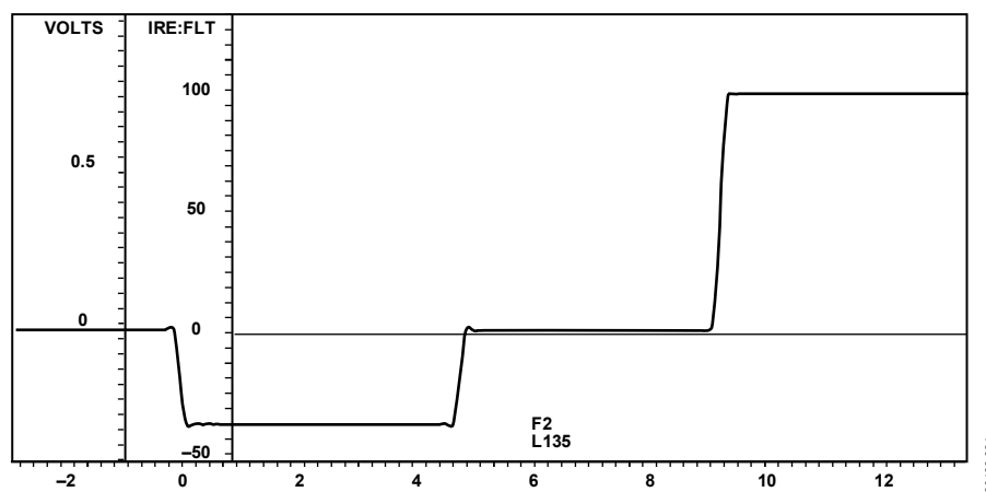
Figure 82. Example of Video Output with Subaddress 0x82, Bit 7 = 1
