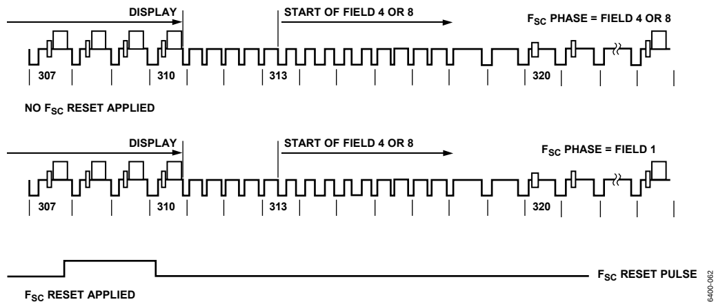
Figure 60. SD Subcarrier Phase Reset Timing Diagram (Subaddress 0x84, Bits[2:1] = 01)
