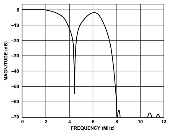
Figure 32. SD PAL, Luma Notch Filter Response
