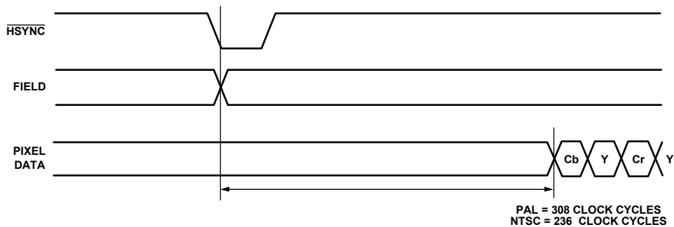
Figure 63. Square Pixel Mode Active Pixel Timing
