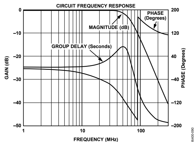
Figure 90. Output Filter Plot for HD, 4x Oversampling
