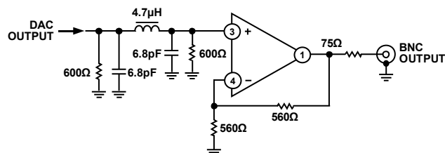
Figure 86. Example of Output Filter for ED, 8 \times Oversampling
