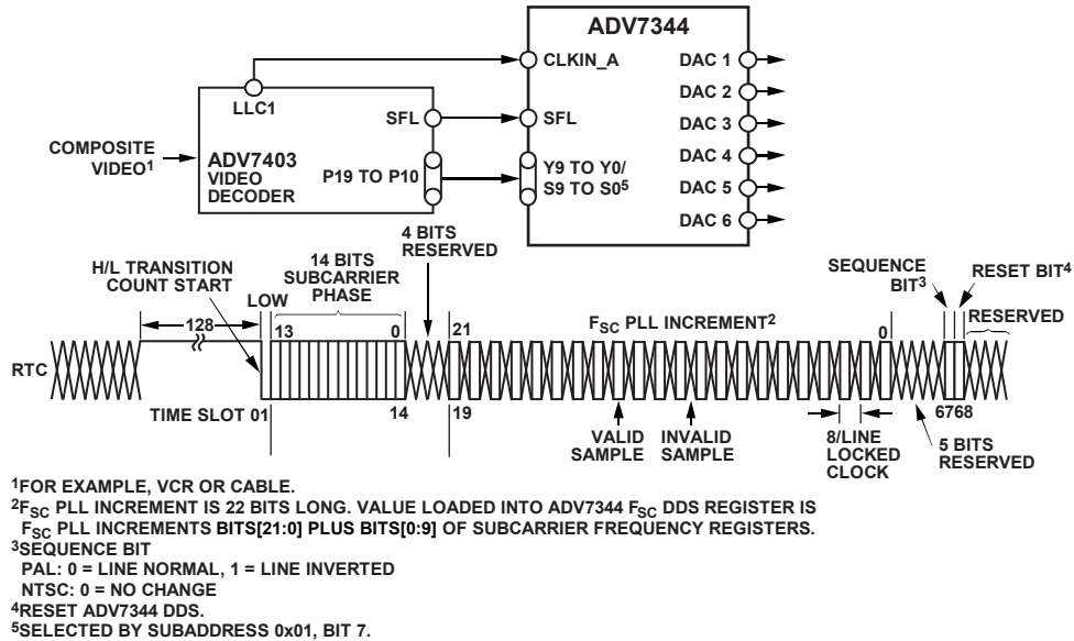
Figure 61. SD Subcarrier Frequency Lock Timing and Connections Diagram (Subaddress 0x84, Bits[2:1] = 11)
