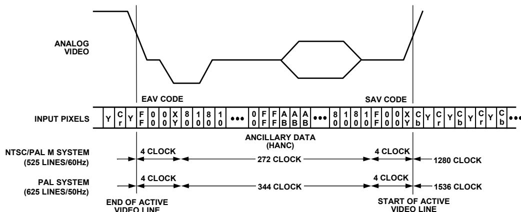
Figure 62. Square Pixel Mode EAV/SAV Embedded Timing
