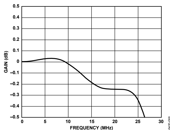
Figure 66. ED/HD Sinc Compensation Filter Disabled
