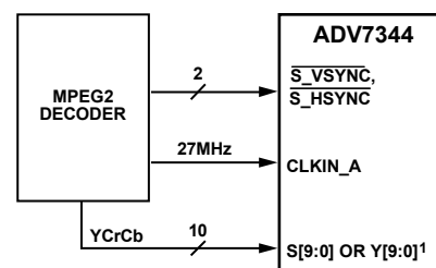
Figure 50. SD Only Example Application
