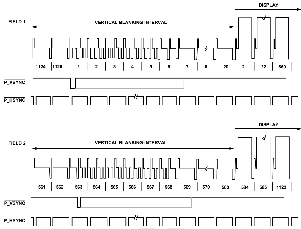
Figure 114. 1080i HSYNC and VSYNC Input Timing
