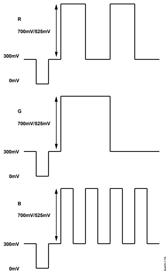
Figure 126. SD/ED RGB Output Levels—RGB Sync Enabled
