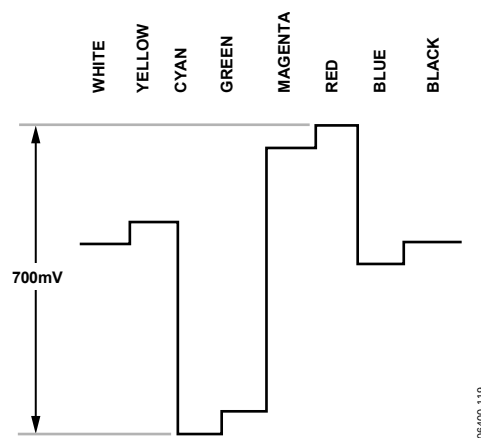
Figure 119. Pr Levels—PAL
