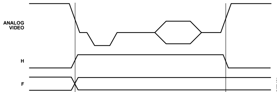
Figure 104. SD Master Mode 0, Data Transitions
