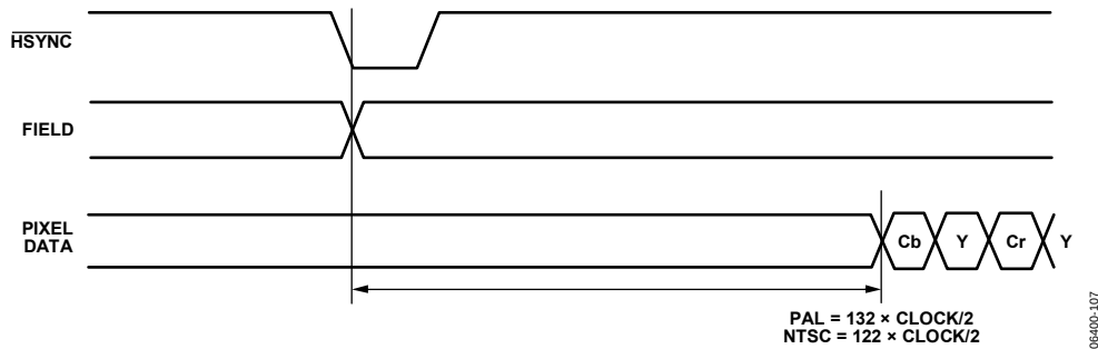
Figure 107. SD Timing Mode 1, Odd/Even Field Transitions (Master/Slave)
