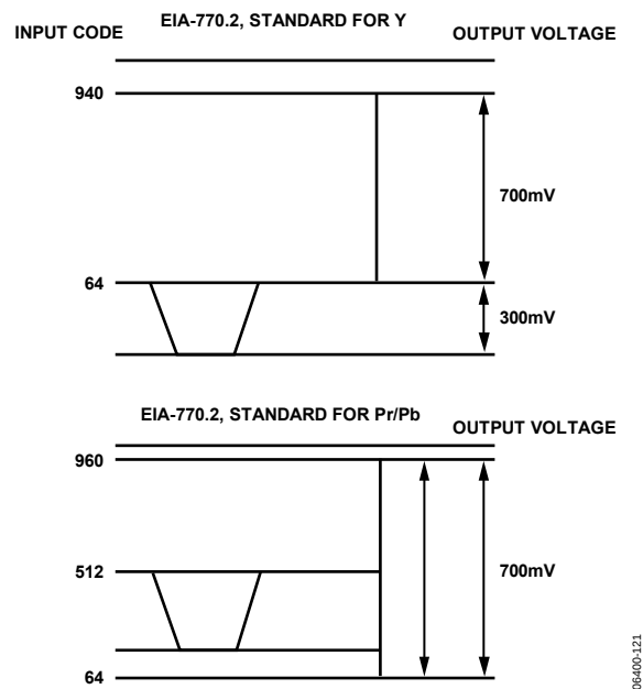
Figure 121. EIA-770.2 Standard Output Signals (525p/625p)
