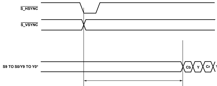
Figure 18. SD Input Timing Diagram (Timing Mode 1)
