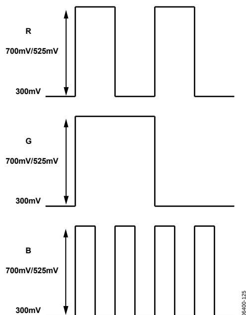
Figure 125. SD/ED RGB Output Levels—RGB Sync Disabled
