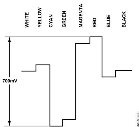
Figure 116. Pr Levels—NTSC
