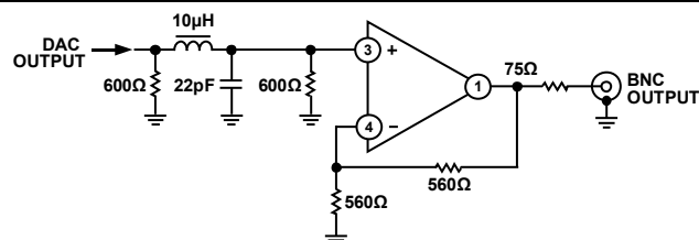
Figure 85. Example of Output Filter for SD, 16 \times Oversampling
