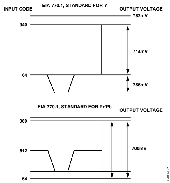
Figure 122. EIA-770.1 Standard Output Signals (525p/625p)
