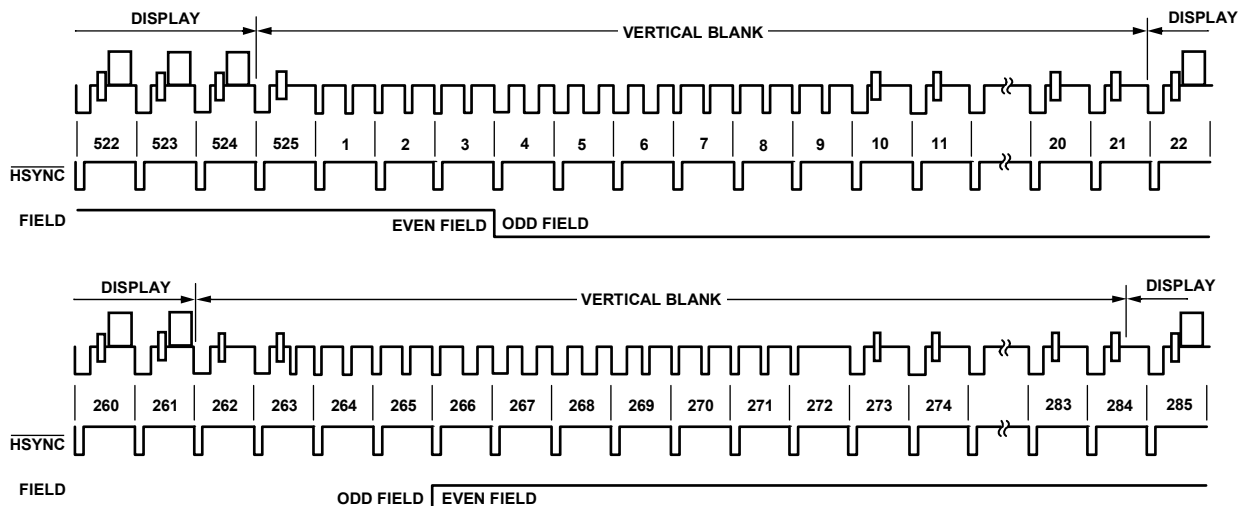
Figure 105. SD Slave Mode 1, NTSC
