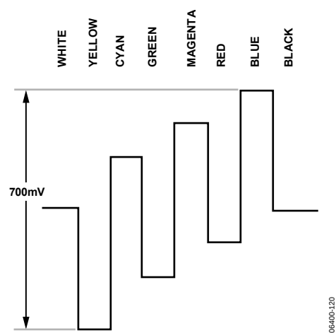
Figure 120. Pb Levels—PAL
