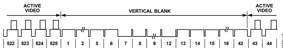
Figure 137. SMPTE 293M (525p)
