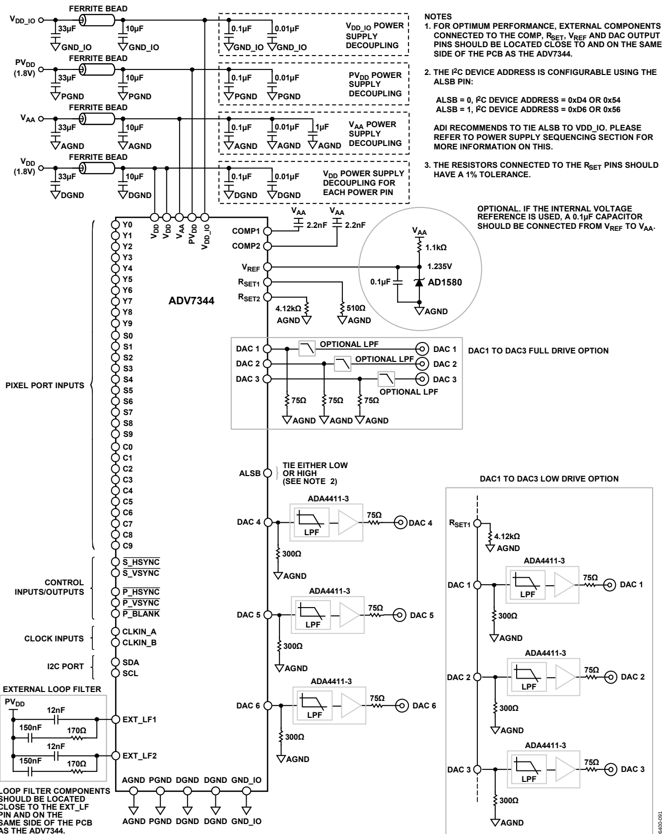
Figure 91. ADV7344 Typical Application Circuit
