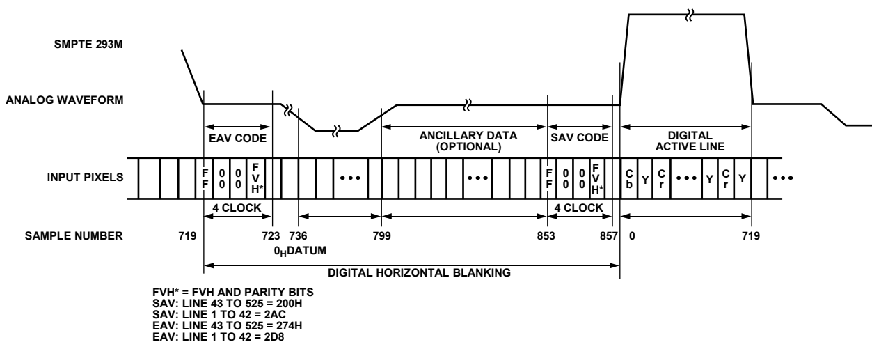
Figure 136. EAV/SAV Input Data Timing Diagram (SMPTE 293M)
