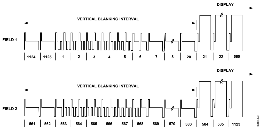
Figure 140. SMPTE 274M (1080i)
