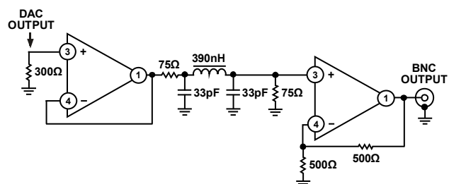
Figure 87. Example of Output Filter for HD, 4 \times Oversampling
