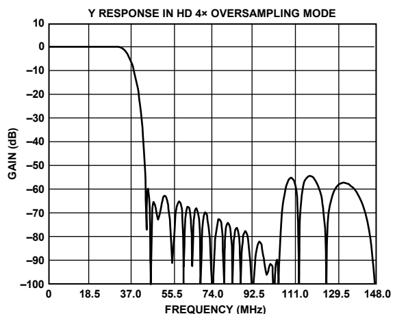
Figure 27. HD 4x Oversampling, Y Filter Response
