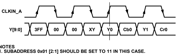
Figure 52. ED/HD-DDR Input Sequence (EAV/SAV)—Option B
