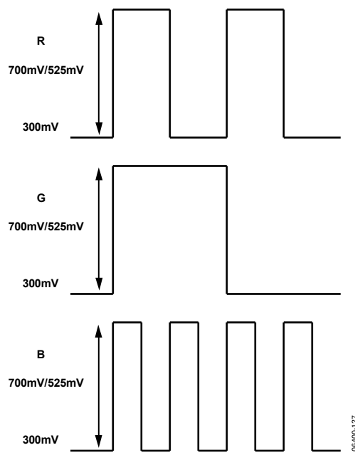
Figure 127. HD RGB Output Levels—RGB Sync Disabled
