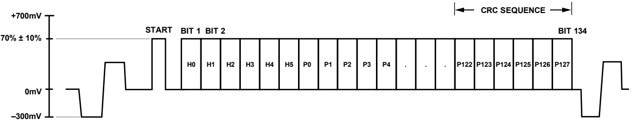
Figure 98. High Definition (720p and 1080i) CGMS Type B Waveform
