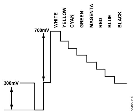
Figure 118. Y Levels—PAL
