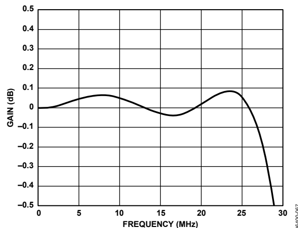
Figure 65. ED/HD Sinc Compensation Filter Enabled
