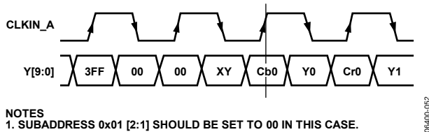
Figure 51. ED/HD-DDR Input Sequence (EAV/SAV)—Option A
