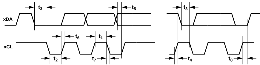
Figure 2. I²C Timing
