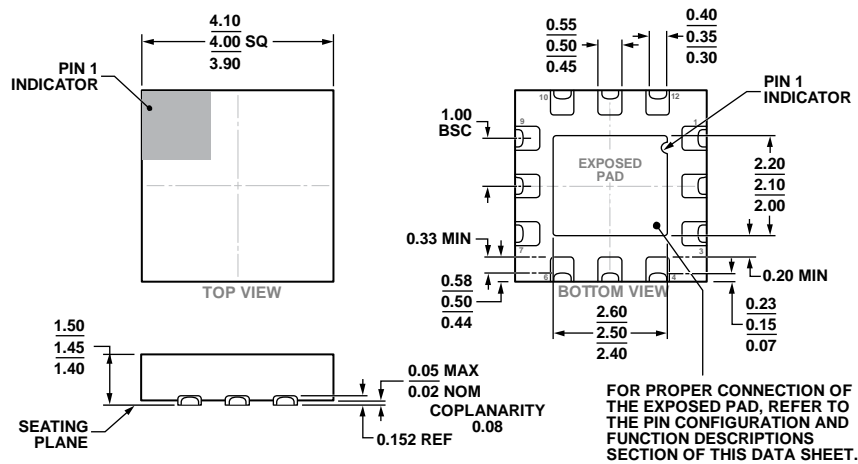
Figure 25. 12-Lead Lead Frame Chip Scale Package [LFCSP_SS] 4 mm × 4 mm Body and 1.45 Package Height, With Side Solderable Leads (CS-12-3) Dimensions shown in millimeters
