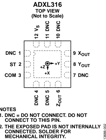
Figure 2. Pin Configuration
