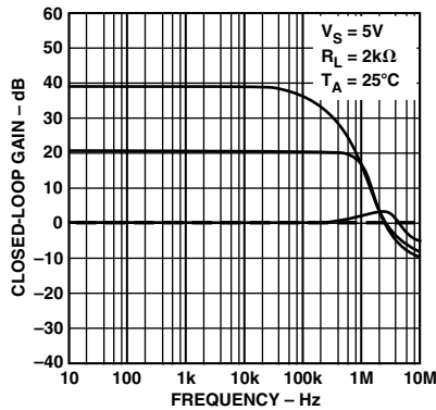
TPC 16. Closed-Loop Gain vs. Frequency (2 kΩ Load)
