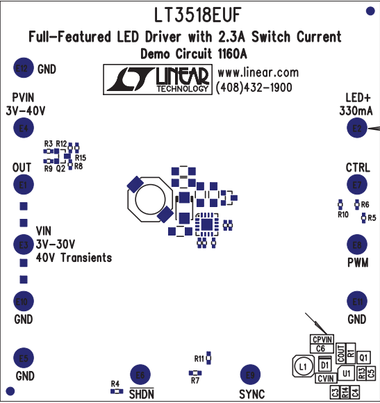
Silkscreen Top
