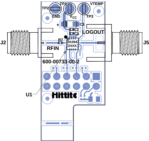
Figure 22. Evaluation PCB Layout, Top Side
