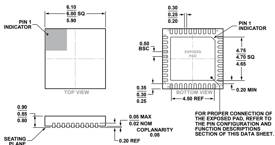
Figure 36. 40-Lead Lead Frame Chip Scale Package [LFCSP] 6 mm × 6 mm Body and 0.85 mm Package Height (HCP-40-1)
