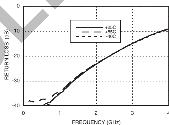
Return Loss
