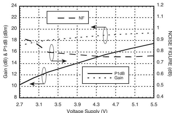
P1dB, Gain, & Noise Figure vs. Supply Voltage @ 2500 MHz
