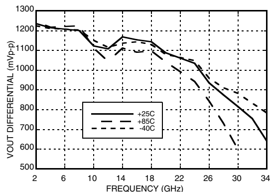
Output Differential Voltage vs. Input Frequency [1][4]
