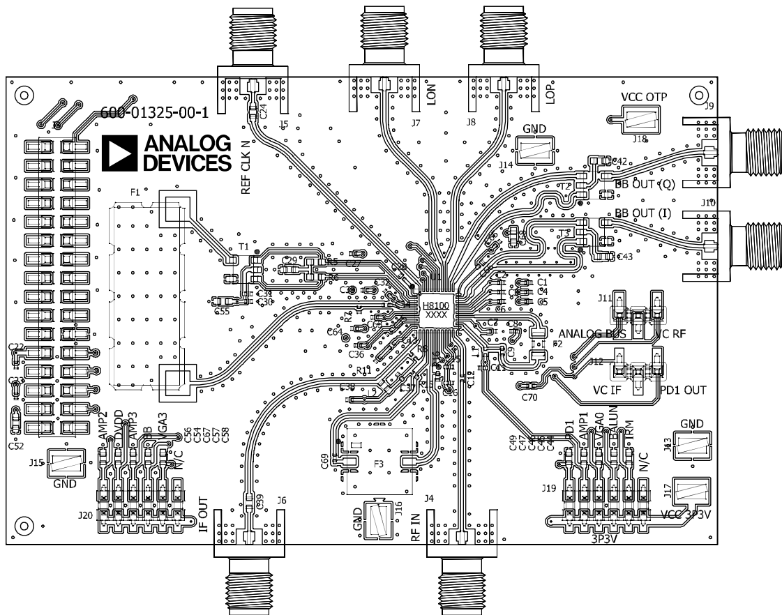
Figure 53. Evaluation PCB
