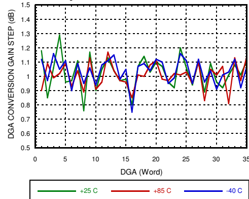
Conversion Gain Step vs. DGA word over Temperature, RF = 4 GHz
