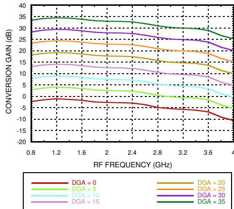
Conversion Gain vs. RF Frequency over DGA Word [1]
