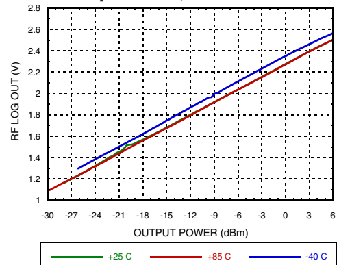
Log RF Detector vs. Output Power over Temperature, RF = 0.8 GHz
