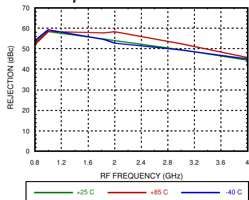
IF to RF Rejection vs. RF Frequency over Temperature [2]
