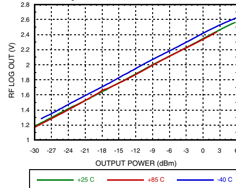
Log RF Detector vs. Output Power over Temperature, RF = 4 GHz
