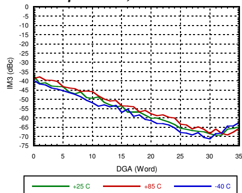
IM3 vs. DGA Word over Temperature, RF = 2 GHz [1]
