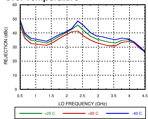
LO to RF Rejection vs. LO Frequency over Temperature [1]
