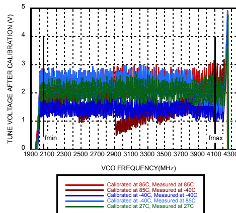
Figure 40. Typical VCO Tuning Voltage After Calibration
