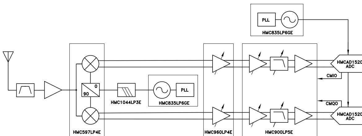
Figure 37. HMC835LP6GE in a typical receive chain
