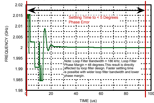
Figure 32. Frequency Settling After Frequency Change, AutoCal Enabled [22]
