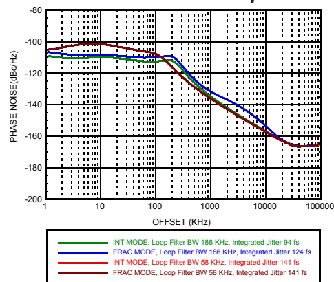
Figure 5. Closed Loop Phase Noise at 3300MHz for different Loop Filter [4][5]
