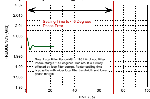
Figure 34. Frequency Settling After Frequency Change, Manual Calibration [23]
