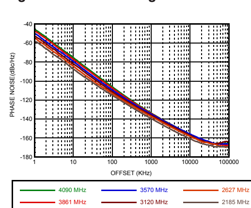
Figure 6. Free Running VCO Phase Noise
