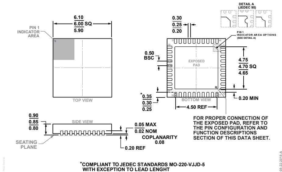
Figure 48. 40-Lead Lead Frame Chip Scale Package [LF CSP] 6 mm × 6 mm Body and 0.85 mm Package Height (HCP-40-1)
