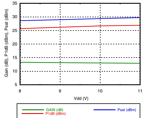
Gain & Power vs. Supply Voltage @ 16 GHz
