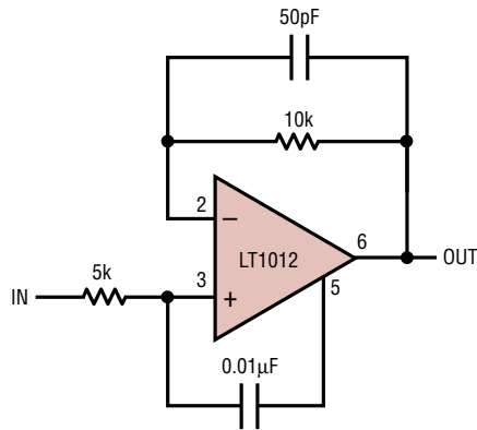
Follower Feedforward Compensation
