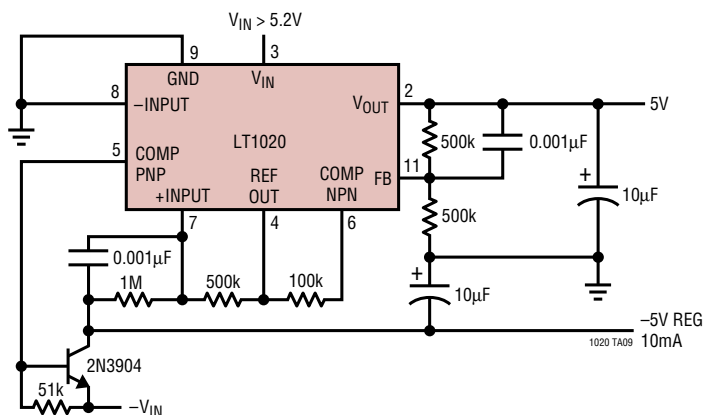
Dual Output Regulator
