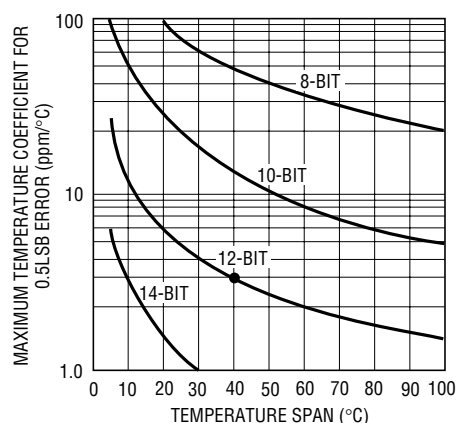
Figure 1. Maximum Allowable Reference Drift
