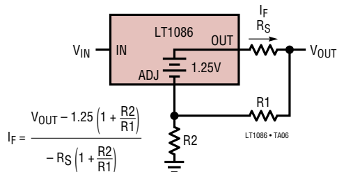
Battery Charger
