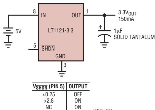
5V Battery-Powered Supply with Shutdown
