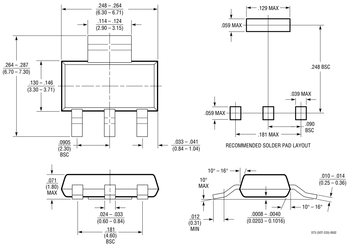
ST Package 8-Lead Plastic SOT-223 (LTC DWG # 05-08-1630)
