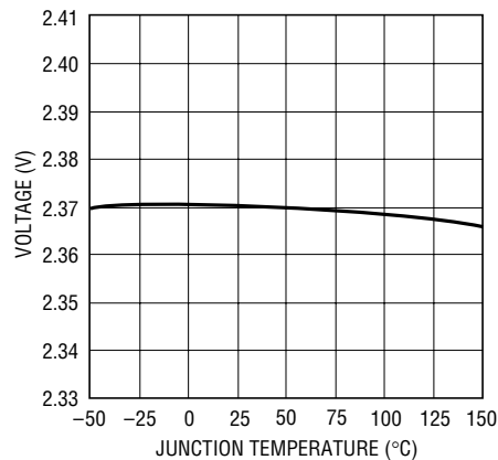
Feedback Pin Voltage Temperature Drift
