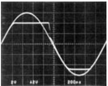
Output Overload
