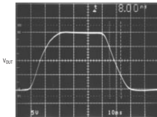
Large-Signal Transient Response, A_V = +10
