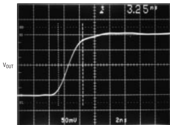
Small-Signal Rise Time, A_V = +2
