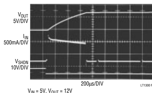
Figure 5. Start-Up Response
