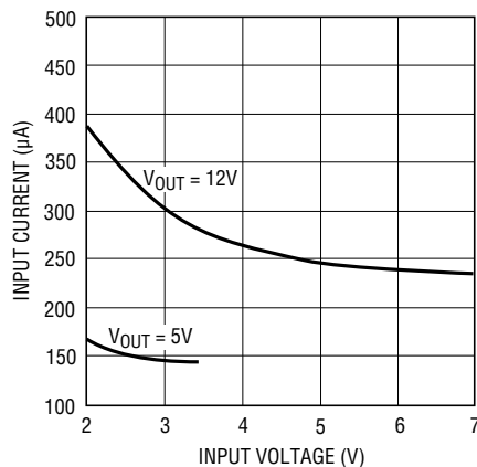
No-Load Input Current
