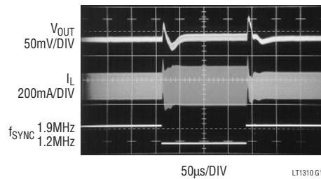
PLL Response
