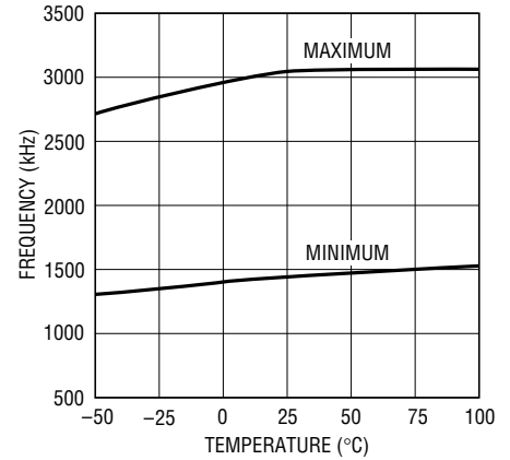
PLL Lock Range 47pF Capacitor on C_T Pin
