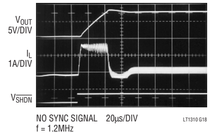
Start-Up Response
