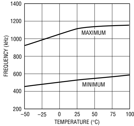
PLL Lock Range 220pF Capacitor on C_T Pin
