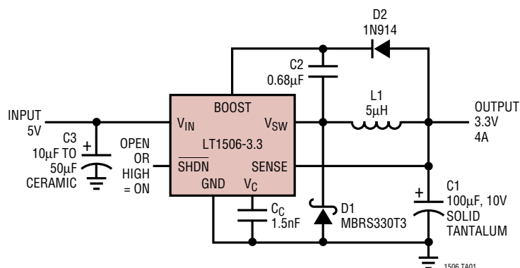
5V to 3.3V Down Converter
