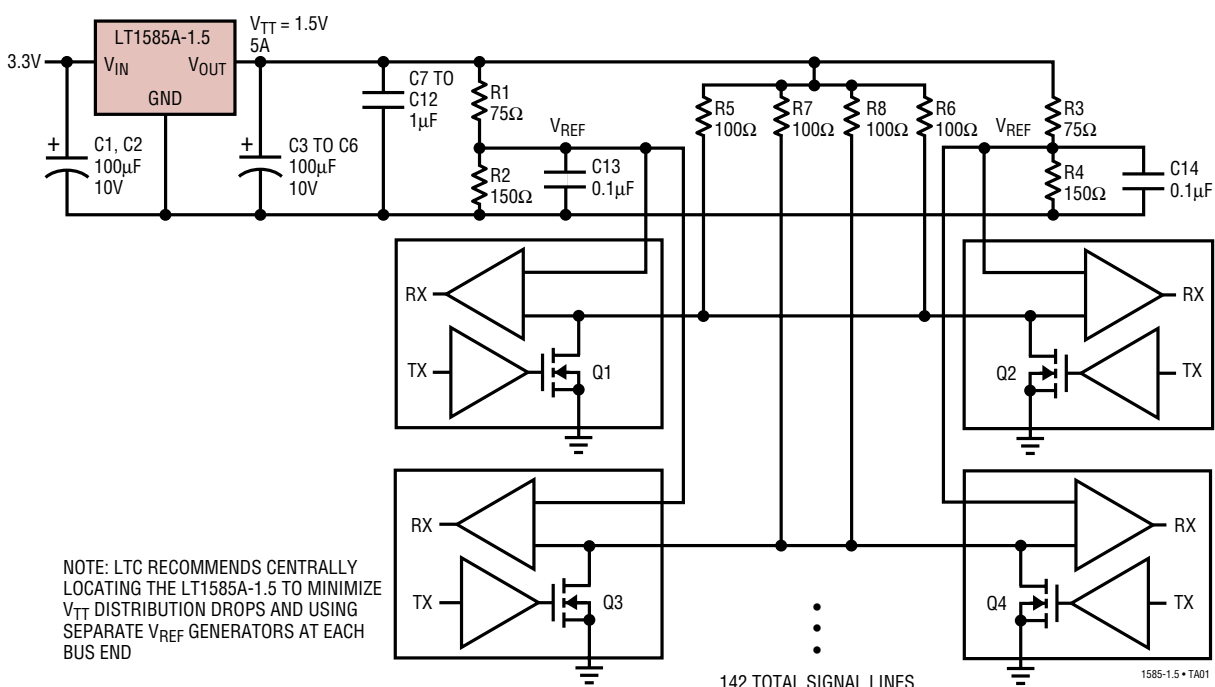
Intel Processor GTL+ Supply
