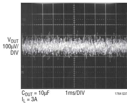
LT1764-3.3 10Hz to 100kHz Output Noise
