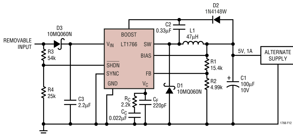
Figure 12. Dual Source Supply with 25\mu A Reverse Leakage
