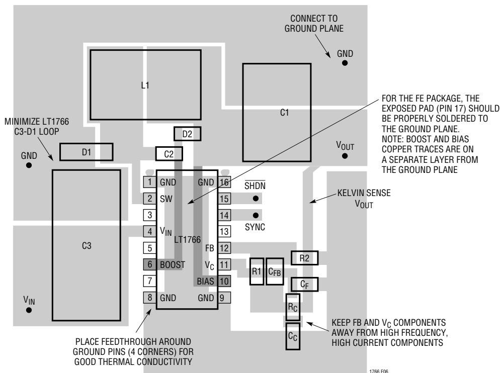
Figure 6. Suggested Layout
