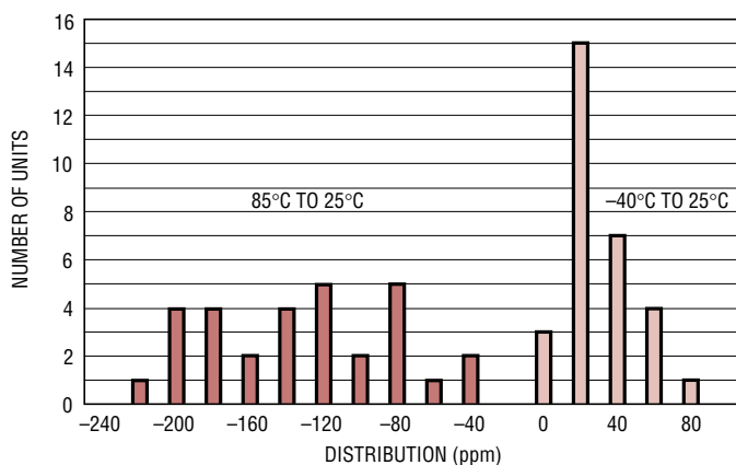
Figure 9. Worst-Case -40°C to 85°C Hysteresis on 30 Units
