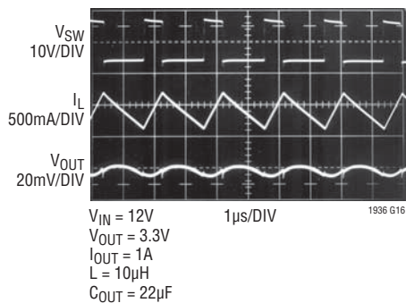
Switching Waveforms
