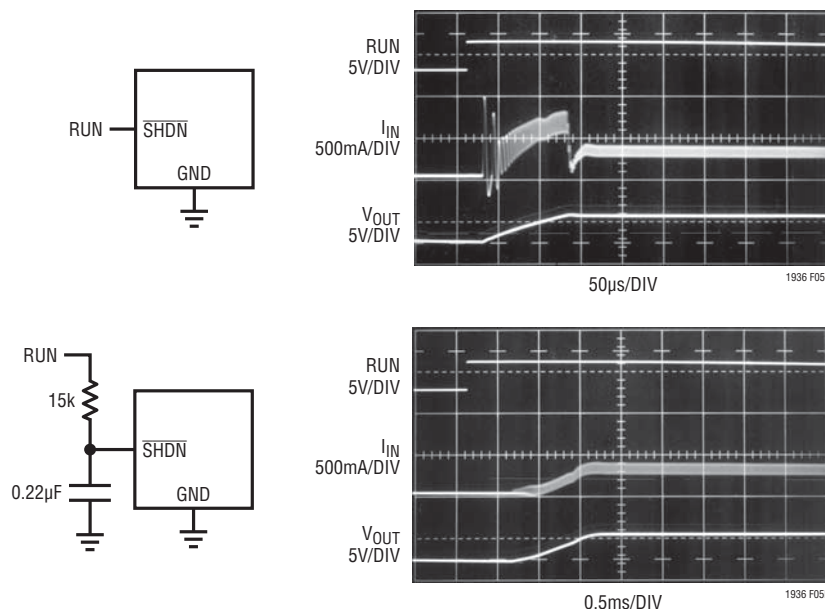
Figure 5. To Soft-Start the LT1936, Add a Resistor and Capacitor to the \overline{\text{SHDN}} Pin. V_{IN} = 12\text{V} , V_{OUT} = 3.3\text{V} , C_{OUT} = 2 \times 22\mu\text{F} , R_{LOAD} = 3.3\Omega
