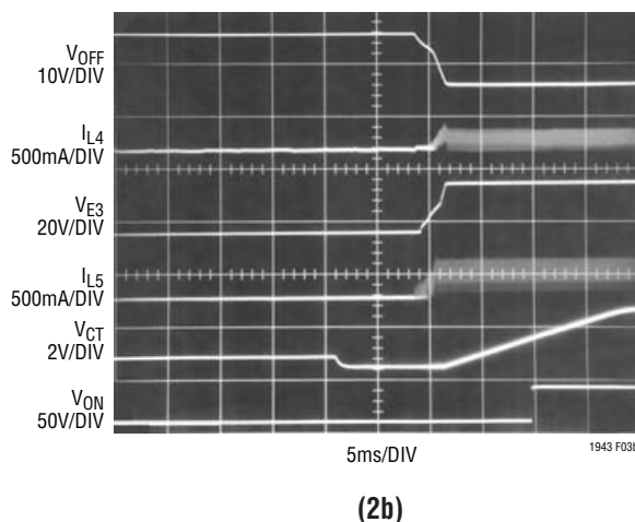
Figure 2. LT1943 Power-Up Sequence. (Traces From Both Photos are Synchronized to the Same Trigger)
