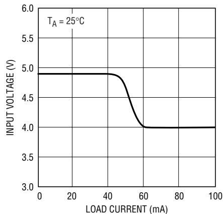
MINIMUM Input Voltage to Start, V_{\text{LOGIC}} = 3.3\text{V}
