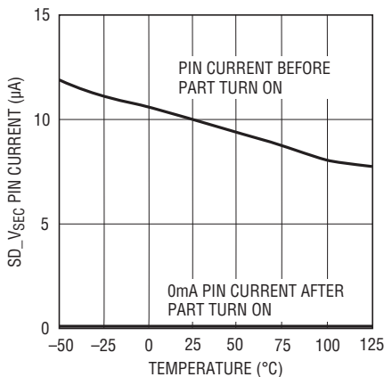
SD\_V_{SEC} Pin Current vs Temperature
