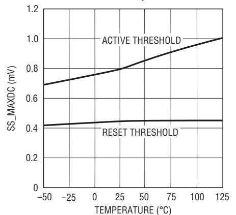
SS\_MAXDC Reset and Active Thresholds vs Temperature
