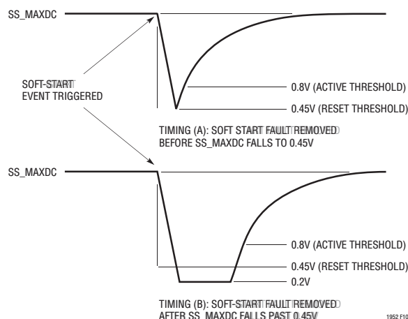
Figure 10. Soft-Start Timing
