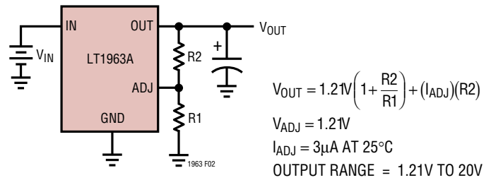
Figure 2. Adjustable Operation
