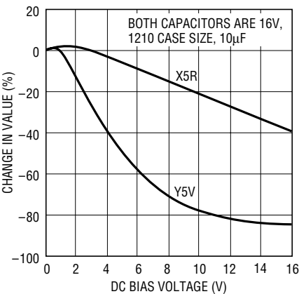
Figure 10. Ceramic Capacitor DC Bias Characteristics
