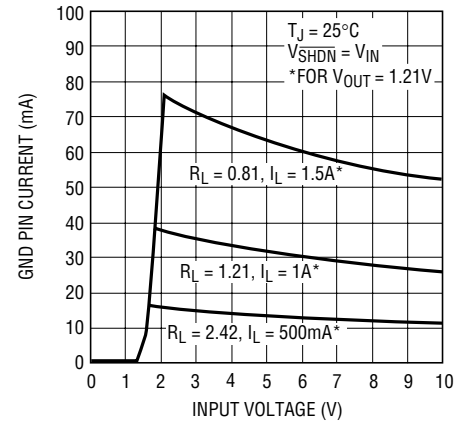
LT1963A GND Pin Current
