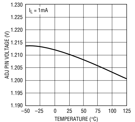
LT1963 ADJ Pin Voltage
