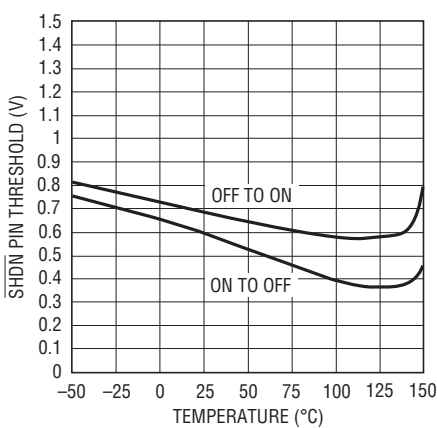
SHDN Pin Thresholds
